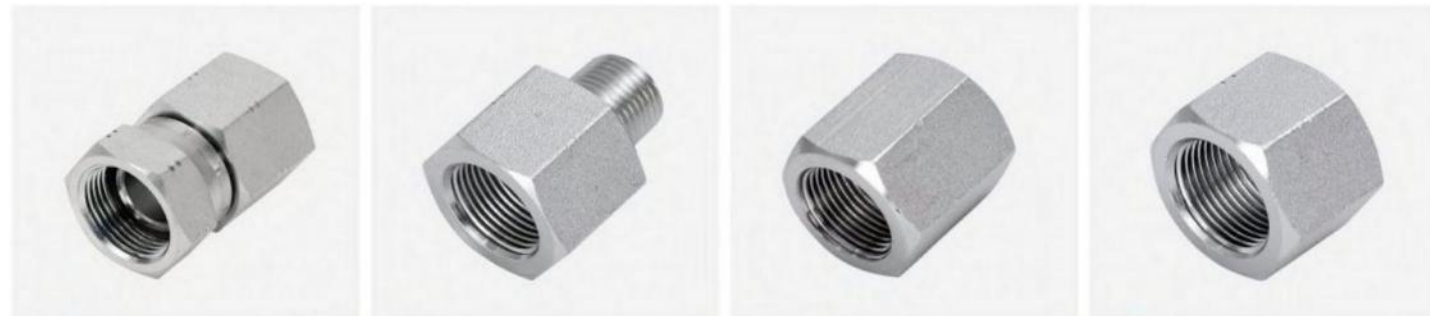
P/N:3NU NPT female / NPSM female 60° cone P/N:5N NPT male / NPT female P/N:7N NPT female P/N:9N NPT female plug
